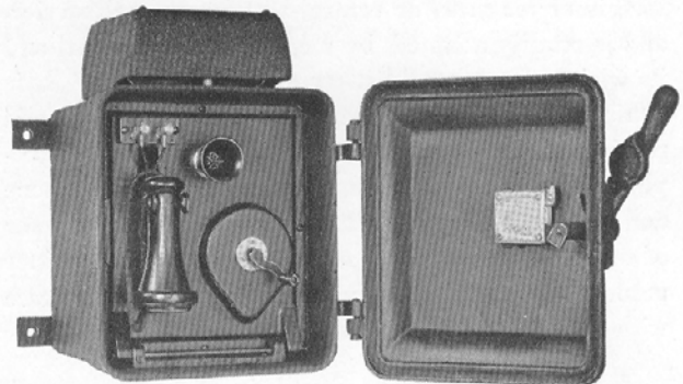
Magneto Mine-Type Telephone Cat. Nos. AM-32 and AM-33
