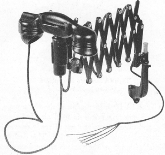
Bracket Monophone, Cat. No. AM-31
