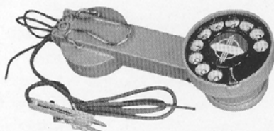
Hand Test Telephone Cat. No. TA-10
